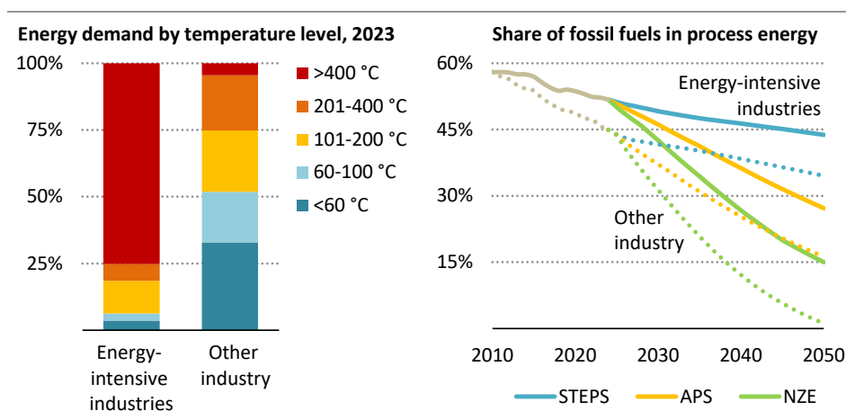
Figure 3.16 ▶ Energy demand by temperature level and fossil fuel use in industry by type and scenario, 2010-2050
